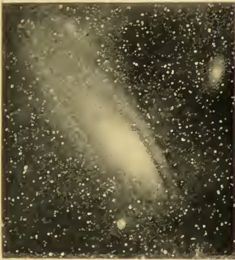
FIG. 88.—The Andromeda Nebula.
